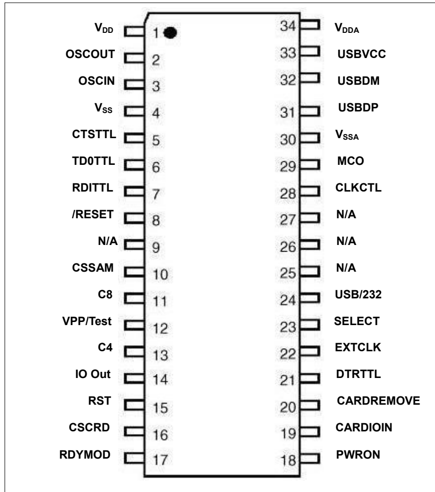
Figure 1. 34-Pin SOIC for AC1030
