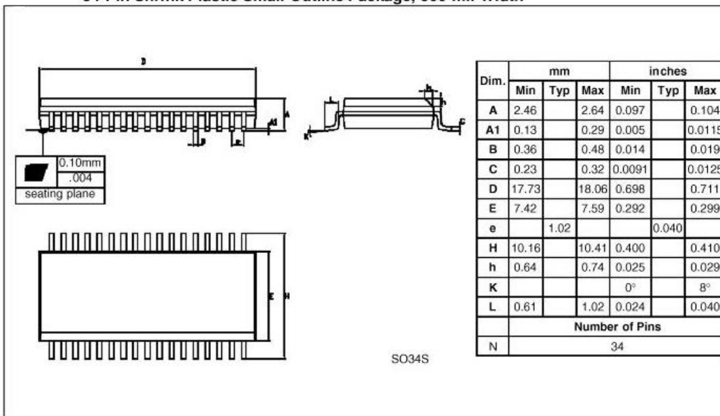
Figure 4. Package Drawing
